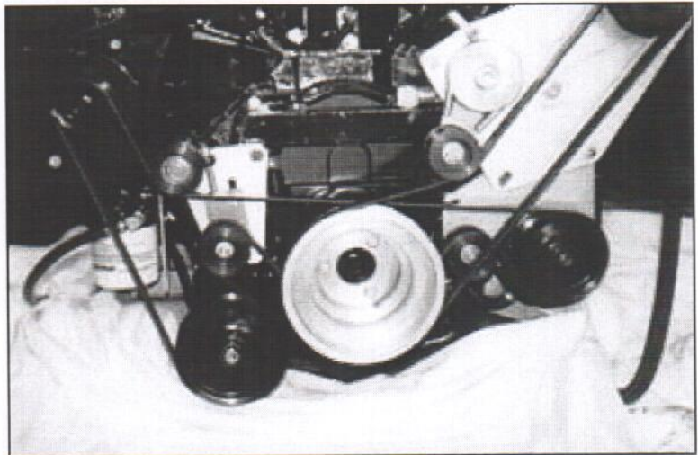
FIGURE D9 ACCESSORY BELT ROUTING
