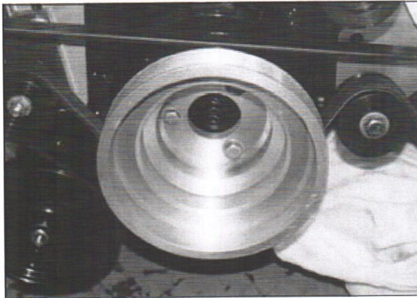
FIGURE B2 CRANK PULLEY INSTALLATION
