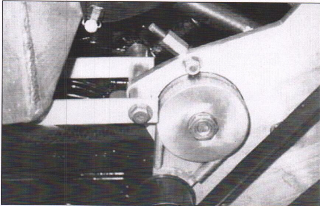
FIGURE D10 PORT SIDE INTERCOOLER TABS MOUNTED TO MAIN BRACKET AND HEAD.
