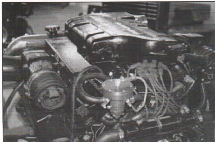
FIGURE G3 FUEL PRESSURE REGULATOR INSTALLATION (1998 ONLY)
