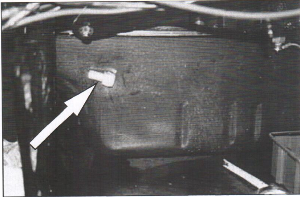
FIGURE A1 OIL DRAIN FITTING LOCATION AND ORIENTATION FITTING SHOULD POINT FORWARD, ANGLED SLIGHTLY UPWARD
