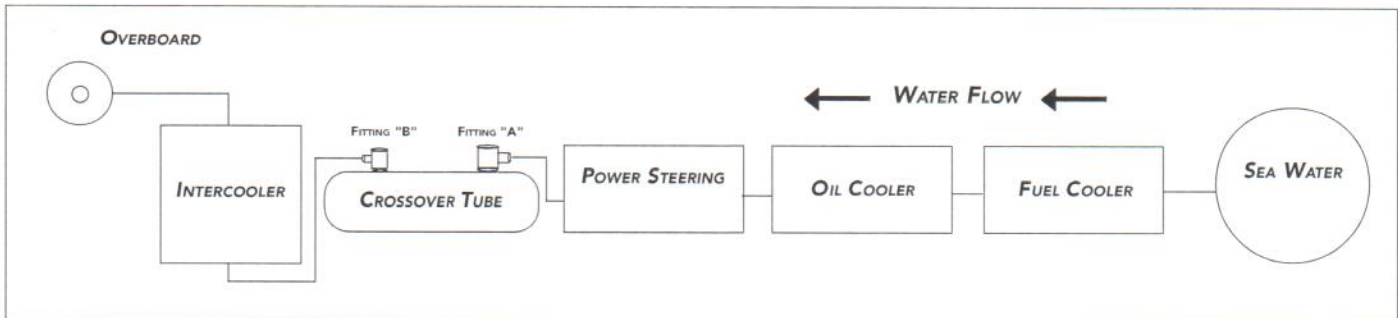
FIGURE F2 TYPICAL WATER ROUTING (NOTE: COOLER SEQUENCE WILL VARY BY BOAT)
