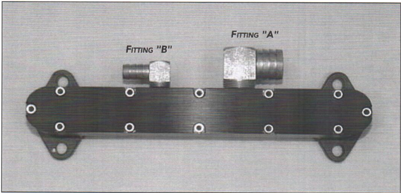
FIGURE F1 CROSSOVER TUBE/WATER TEE FITTING
