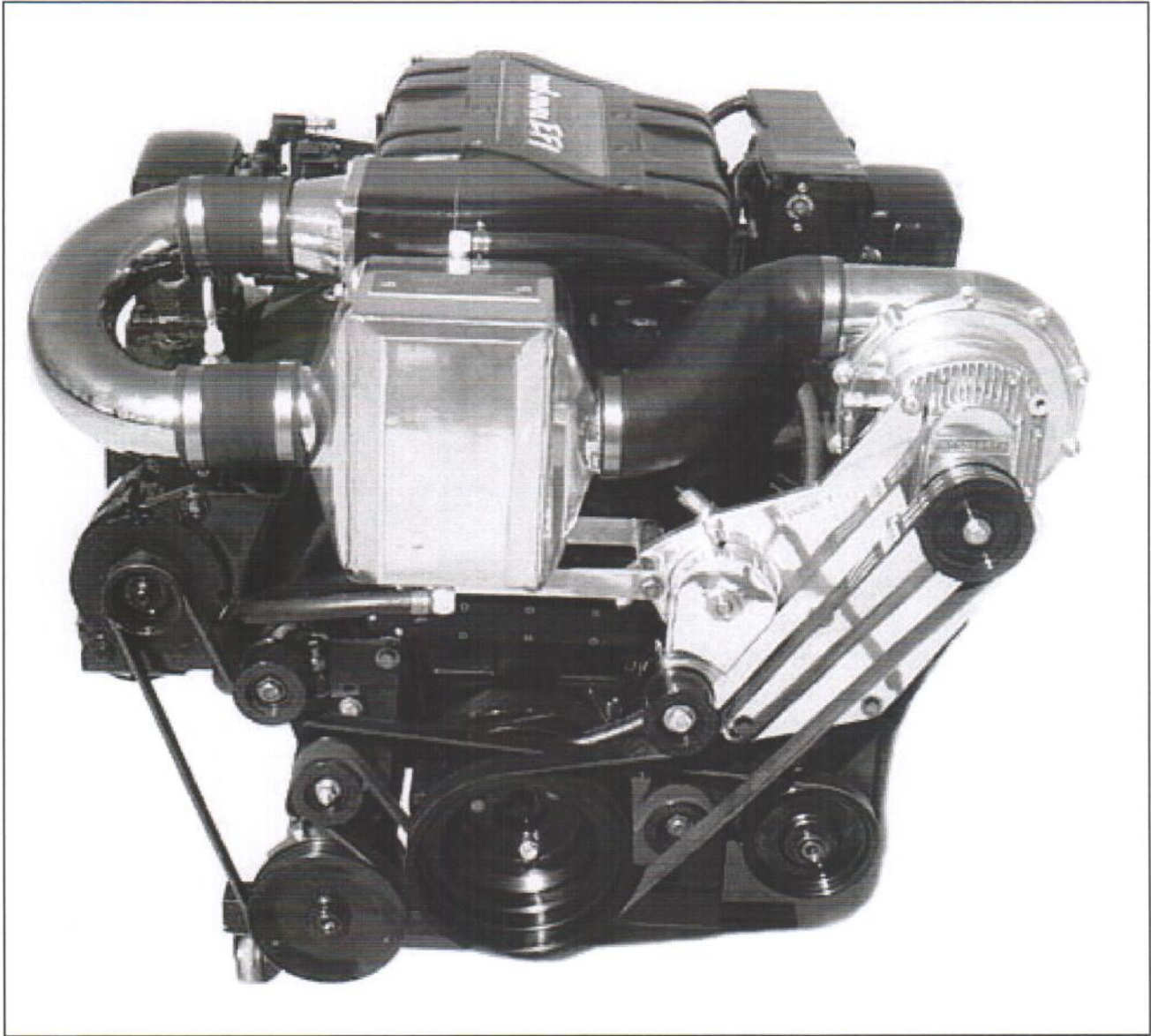
FIGURE H1 COMPLETED ProCHARGER SYSTEM INSTALLATION
