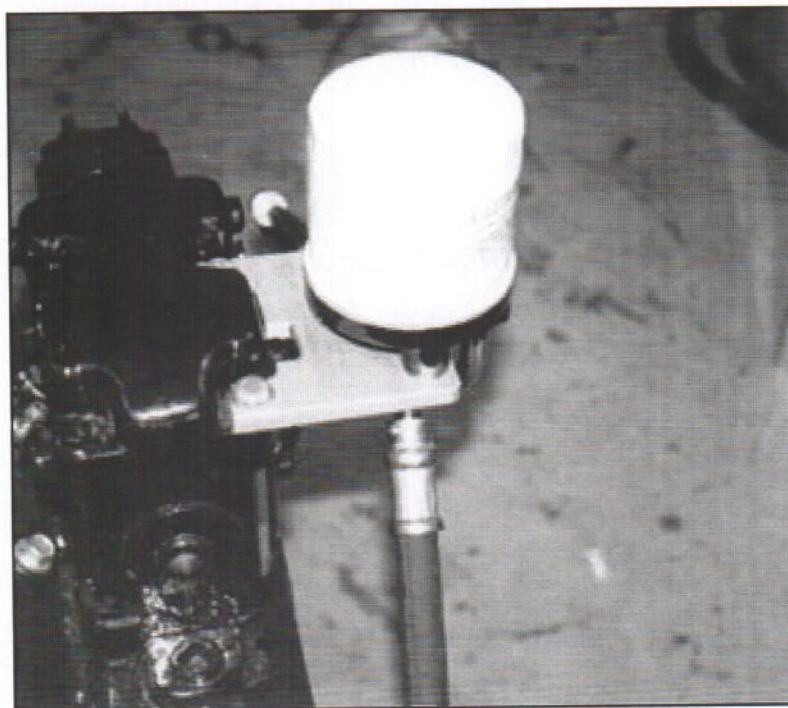
FIGURE C1 OIL FILTER BRACKET INSTALLATION
