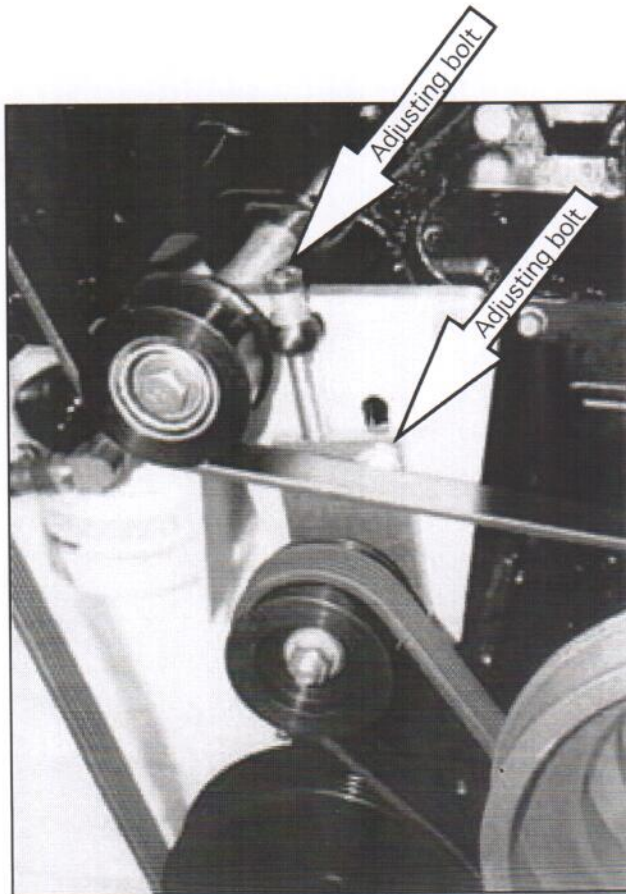
FIGURE D8 TENSIONER-BRACKET ADJUSTING BOLTS
