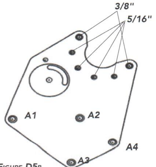
SC MAIN BRACKET ORIENTATION
