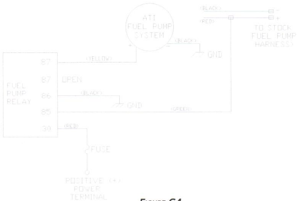
FIGURE G4 FUEL PUMP RELAY WIRING DIAGRAM ('97 AND NEWER)
