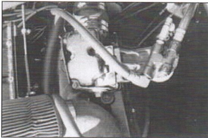
FIGURE C1 OIL FILTER BRACKET INSTALLATION
