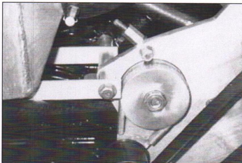
FIGURE D7 PORT SIDE INTERCOOLER TABS MOUNTED TO MAIN BRACKET AND HEAD.
