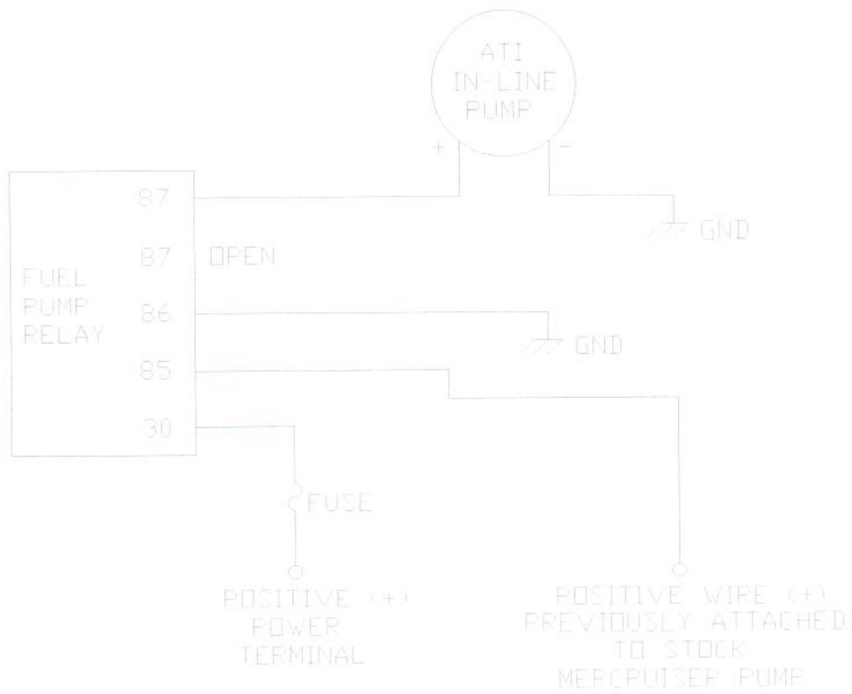
FIGURE G2 FUEL PUMP RELAY WIRING DIAGRAM '96 AND OLDER
