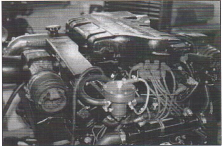
FIGURE G6 FUEL PRESSURE REGULATOR
