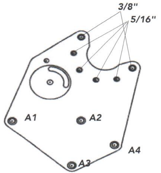
SC BRACKET
